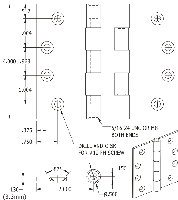
4×4×.130 (3.3mm) INCH SQ HINGE WEIGHT: 0.766LB (347g)
