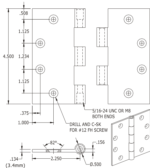
4.5×4.5×.134 (3.4mm) INCH SQ HINGE WEIGHT: 0.957LB (434g)
