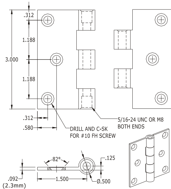
3×3×.092 (2.3mm) INCH SQ HINGE WEIGHT: 0.346LB (157g)
