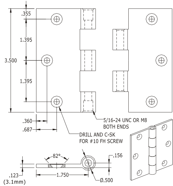
3.5×3.5×.123 (3.1mm) INCH SQ HINGE WEIGHT: 0.564LB (256g)
